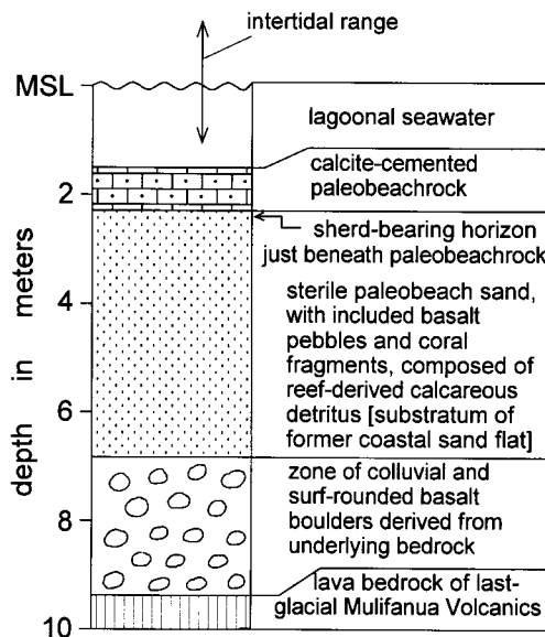
Figure 2. General underwater stratigraphy of the Mulifanua ferry-berth Lapita site (after Jennings, 1974; Green and Richards, 1975; Leach and Green, 1989). MSL = mean sea level.
