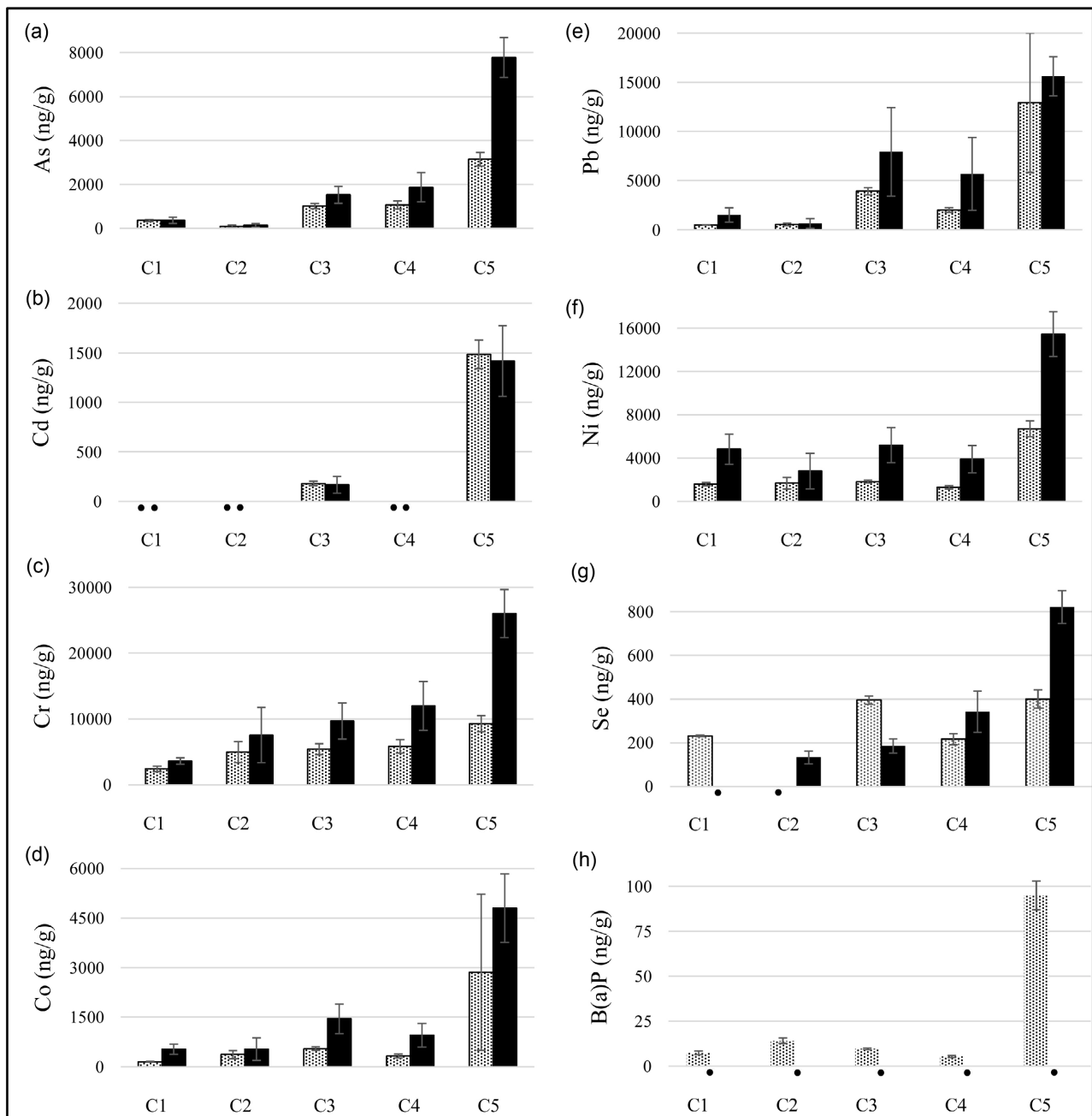
Figure 3. Comparison of trace metals and B[a]P in unburned (gray bars) and burned (black bars) WP charcoal solid waste. (•) means below the limit of quantification. LOQ for As (0.1 µg/L), Cd (0.1 µg/L), Cr (1 µg/L), Co (0.1 µg/L), Pb (0.1 µg/L), Ni (0.1 µg/L), Se (0.5 µg/L), B[a]P (0.5 ng/g).
