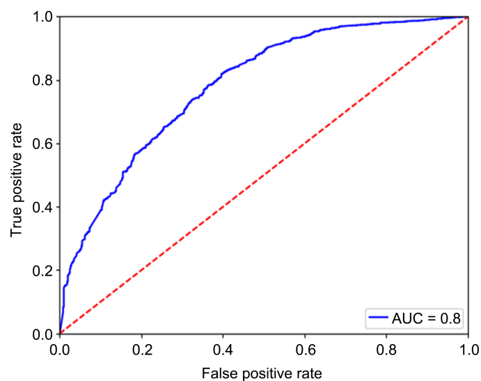
Figure 3. The AUC of the tradapoost (xgboost).
