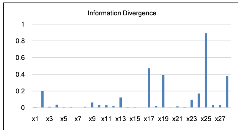
Figure 2. Source domain characteristic information divergence.
