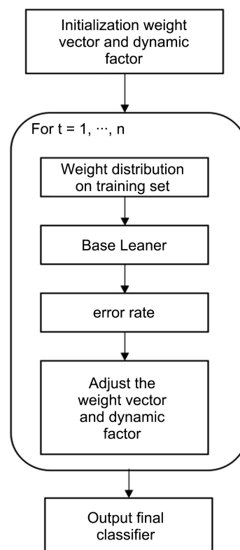
Figure 1. Instance-based TL.
