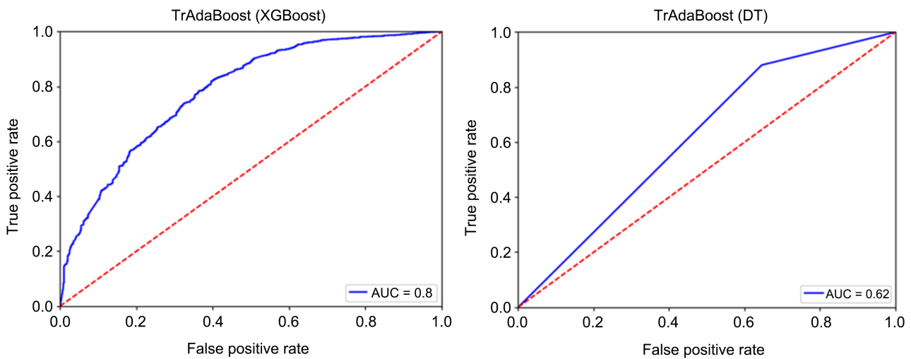
Figure 4. Comparison results-1.
