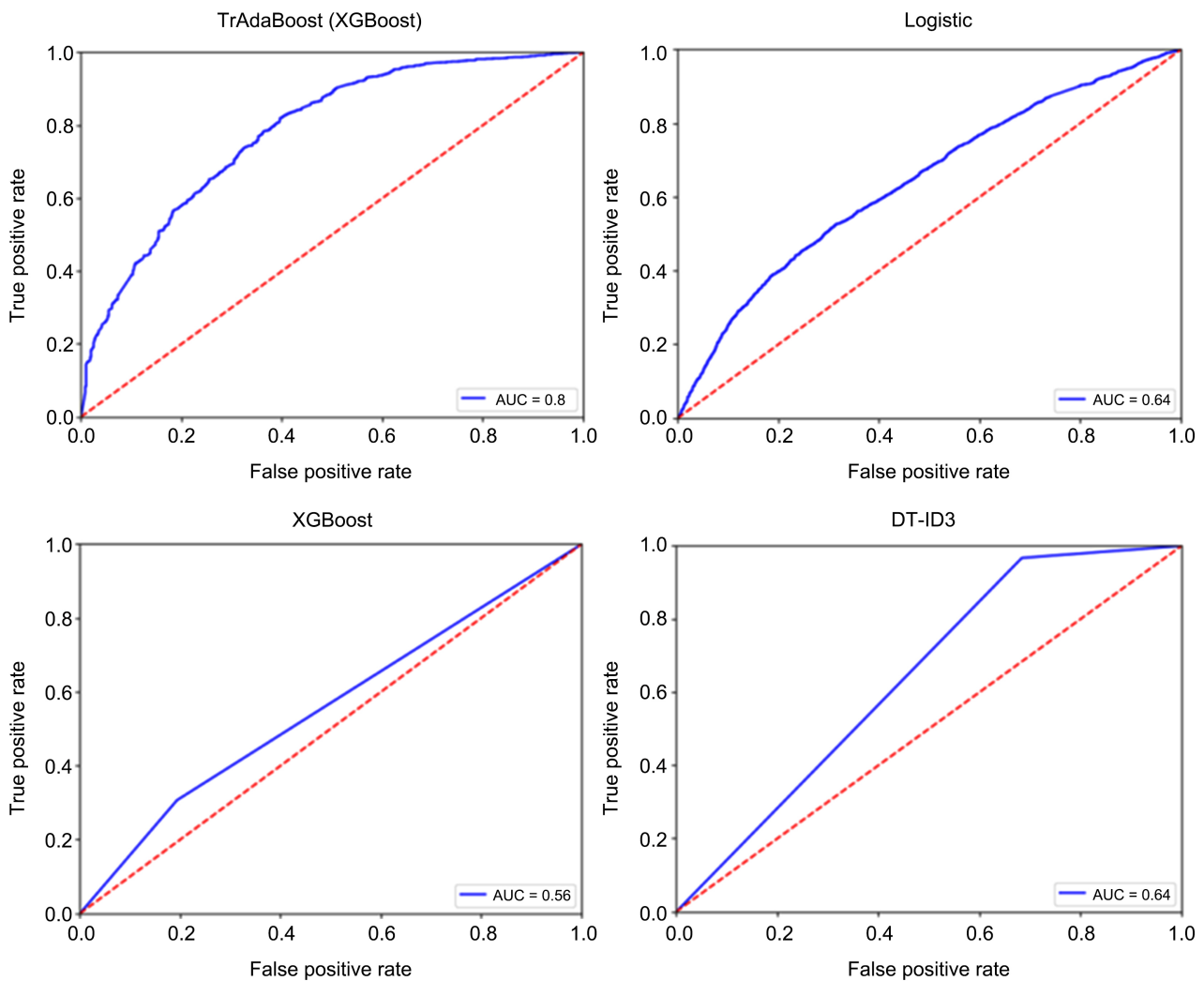
Figure 5. Comparison results-2.
