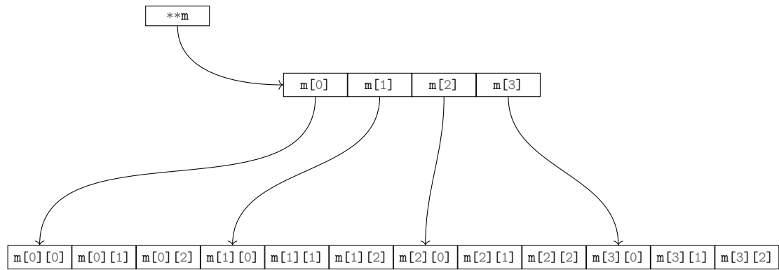
Figure 20.2.: Contiguous Two Dimensional Array. The initial pointer-to-pointers m is initialized to an array of pointers, m[0] . . m[3] . A 4 \times 3 contiguous array is created and each of the pointers is initialized to the proper location so it can be treated as a two-dimensional array.
