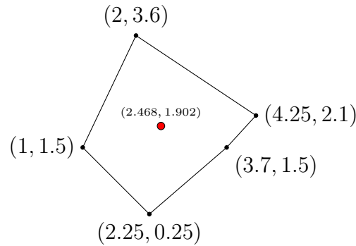
Figure 4.8.: A polygon and its centroid. Whooh!
