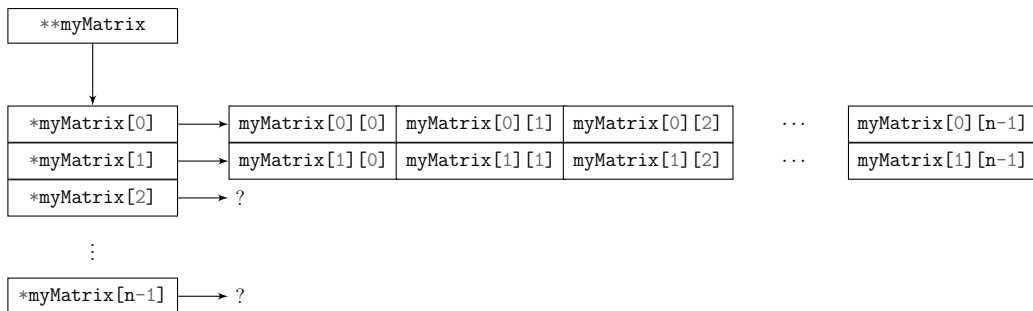
(c) Initialization of the second pointer. On the second iteration of the for loop when i = 1 , the second “row” is initialized.
