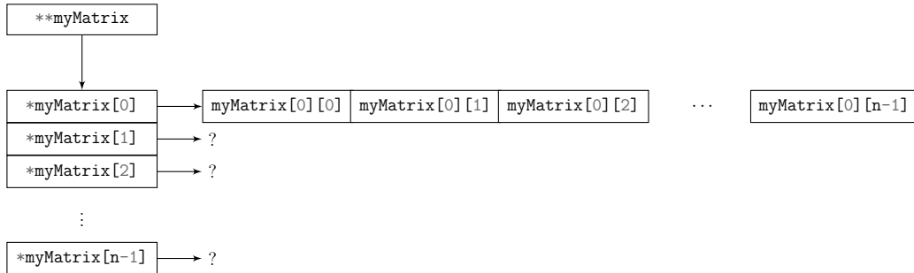
(b) Initialization of the first pointer. On the first iteration of the for loop when i = 0 , the first “row” is initialized when malloc() is invoked.
