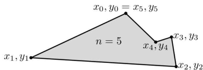
Figure 9.2.: An example polygon for n = 5
