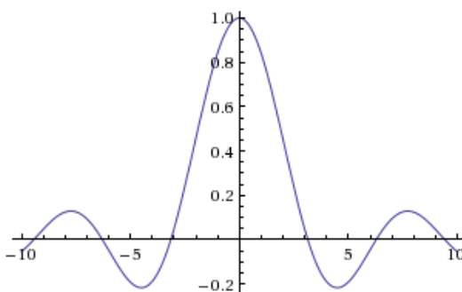
Figure 4.3.: Plot of f(x) = \frac{\sin x}{x}
