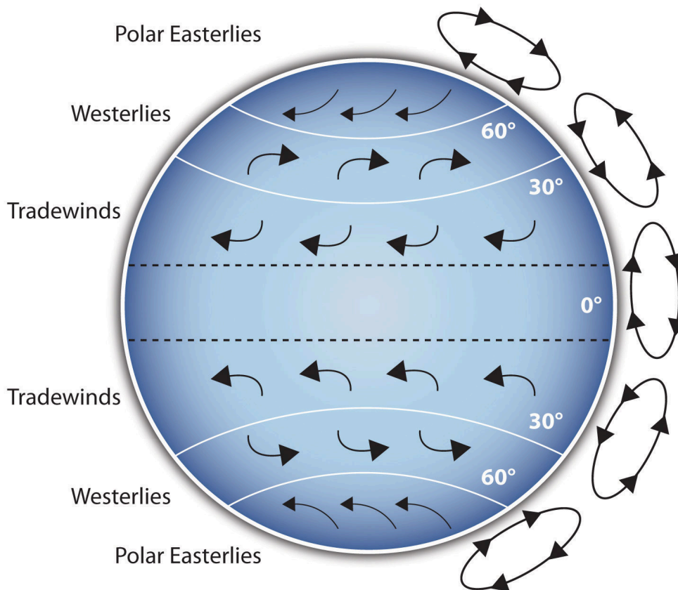
Figure 15.1 Coriolis Effect
